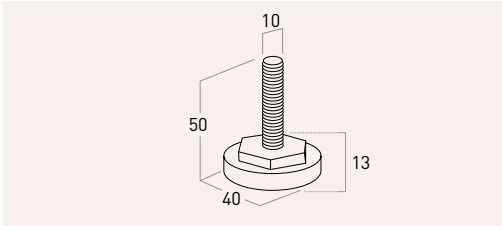
Nivelador Pata ABS Adjuster for ABS Legs
