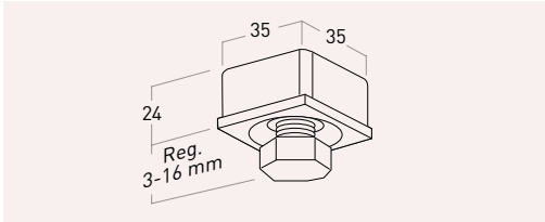
Nivelador Pata ABS Adjuster for ABS Legs
